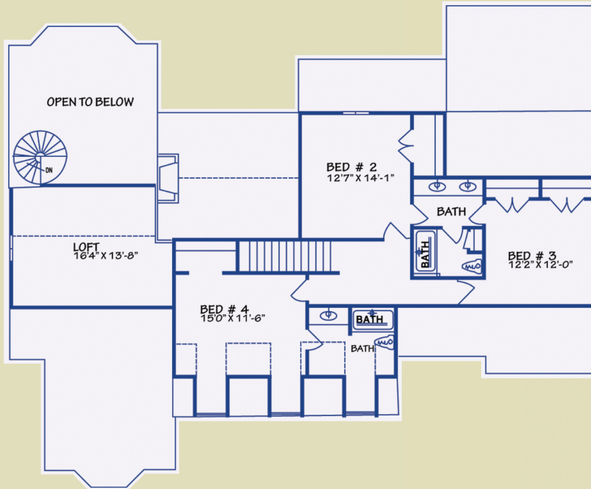
Second Floor
